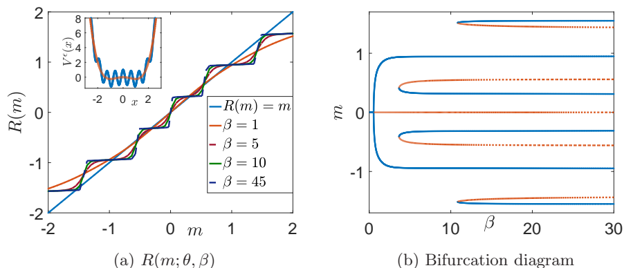
Figure 8: Results for case 3: bistable V_0^b with separable fluctuations, for \theta = 5 , \delta = 1 , \epsilon = 0.1 . (8a) R(m^\epsilon; \theta, \beta) for various values of \beta , with the potential V^\epsilon(x) (full line) compared with V_0^b(x) (dashed line) in the inside panel. (8b) Bifurcation diagram of m as a function of \beta . Full lines correspond to stable solutions, while dashed lines represent unstable ones.
