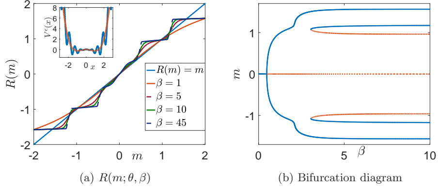
Figure 9: Results for case 4: bistable V_0^b with nonseparable fluctuations, for \theta = 5 , \delta = 1 , \epsilon = 0.1 . (9a) R(m^\epsilon; \theta, \beta) for various values of \beta , with the potential V^\epsilon(x) (full line) compared with V_0^b(x) (dashed line) in the inside panel. (9b) Bifurcation diagram of m as a function of \beta . Full lines correspond to stable solutions, while dashed lines represent unstable ones.
