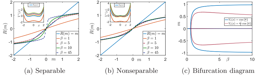
Figure 5: Plot of R(m; \theta, \beta) compared to the diagonal y = x ( R(m; \theta, \beta) = m ) for \theta = 5, \delta = 1, a = 5 and various values of \beta for the homogenized bistable potentials with (5a) separable fluctuations (potentials for various values of \beta shown on the inside panel), and (5b) nonseparable fluctuations (potentials for various values of \beta shown on the inside panel). (5c) Bifurcation diagram of m as a function of \beta for the potentials in (5a) (full line) and (5b) (dashed line).
