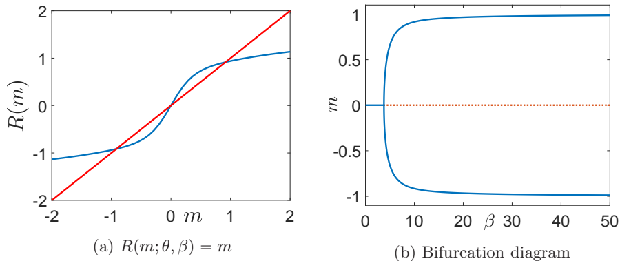
Figure 1: (1a) Plot of R(m; \theta, \beta) and of the straight line y = x for \theta = 0.5 , \beta = 10 , and (1b) bifurcation diagram of m as a function of \beta for \theta = 0.5 for the bistable potential V(x) = \frac{x^4}{4} - \frac{x^2}{2} and interaction potential F(x) = \frac{x^2}{2} .
