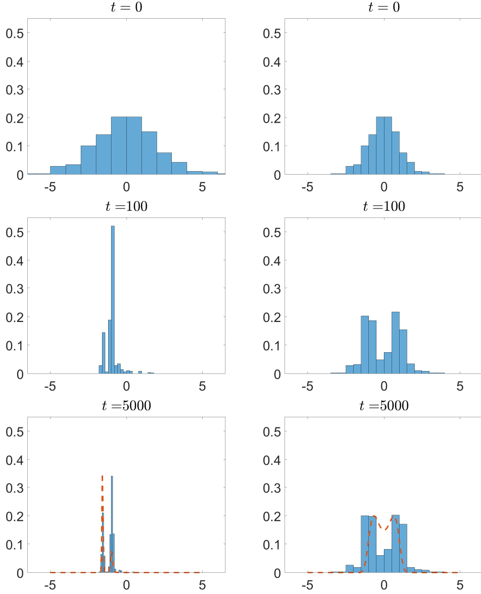
Figure 15: Histogram of N = 500 particles for V^\epsilon(x) = \frac{x^4}{4} - \frac{x^2}{2} (1 - \delta \cos(\frac{x}{\epsilon})) , with \theta = 0.5 , \beta \approx 5.6 , \delta = 1 . Left: Eqn. (2.1) with \epsilon = 0.1 . Right: homogenized SDEs (2.17).
