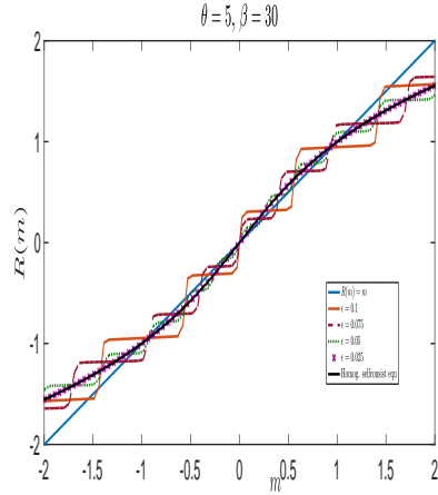
(b) V^\epsilon(x) = \frac{x^4}{4} - \left(1 + \delta \cos\left(\frac{x}{\epsilon}\right)\right) \frac{x^2}{2}
