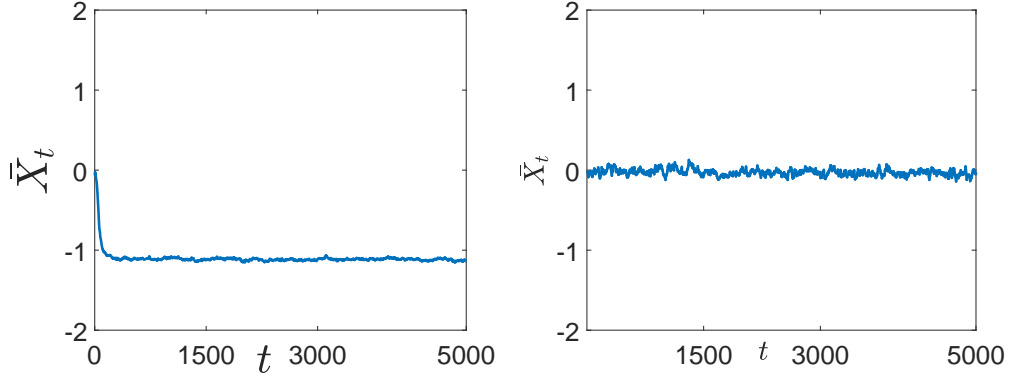
Figure 16: Time evolution of the average \bar{X}_t^N = \frac{1}{N} \sum_{i=1}^N X_t^i of N = 500 particles for V^\epsilon(x) = \frac{x^4}{4} - \frac{x^2}{2} (1 - \delta \cos(\frac{x}{\epsilon})) , with \theta = 0.5 , \beta \approx 5.6 , \delta = 1 . Left: Eqn. (2.1) with \epsilon = 0.1 . Right: homogenized SDEs (2.17).
