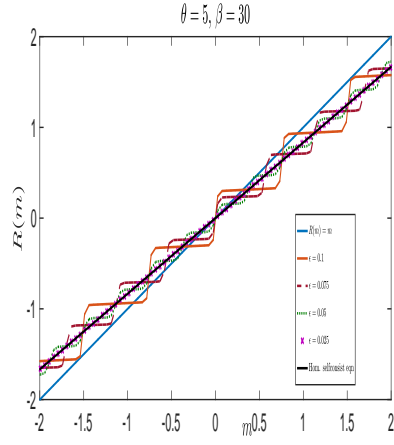
(a) V^\epsilon(x) = \frac{x^2}{2} + \delta \cos\left(\frac{x}{\epsilon}\right)
