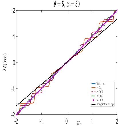
(a) V^\epsilon(x) = \left(1 + \delta \cos\left(\frac{x}{\epsilon}\right)\right) \frac{x^2}{2}
