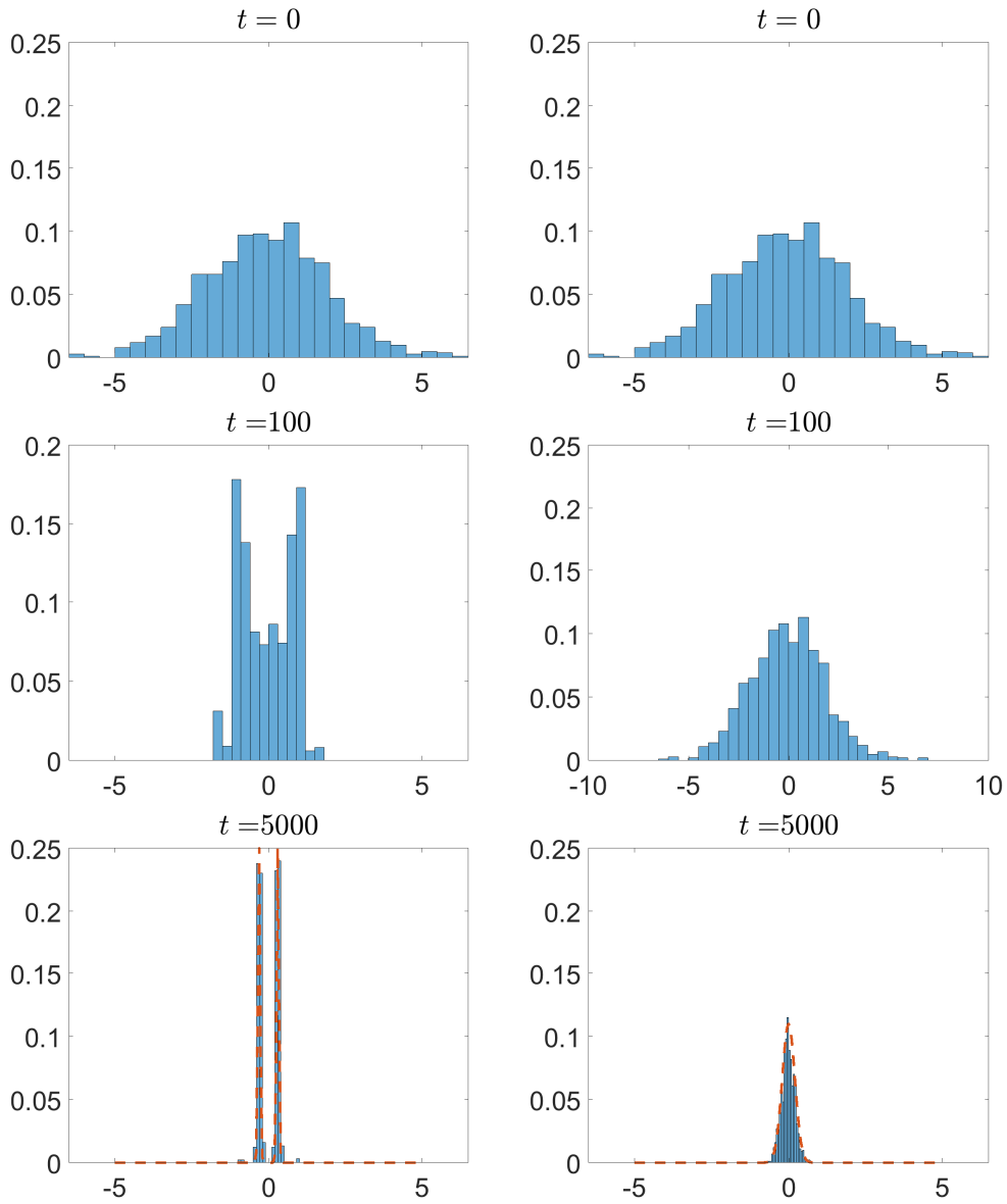
Figure 12: Histogram of N = 1,000 particles for V^\epsilon(x) = \frac{x^2}{2} + \delta \cos\left(\frac{x}{\epsilon}\right) , with \theta = 2 , \beta = 8 , \delta = 1 . Left: Eqn. (2.1) with \epsilon = 0.1 . Right: homogenized SDEs (2.17).
