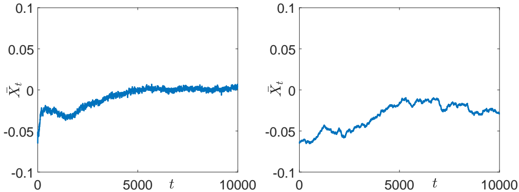
Figure 13: Time evolution of the mean \bar{X}_t^N = \frac{1}{N} \sum_{i=1}^N X_t^i of N = 1,000 particles for V^\epsilon(x) = \frac{x^2}{2} + \delta \cos\left(\frac{x}{\epsilon}\right) , with \theta = 2 , \beta = 8 , \delta = 1 . Left: Eqn. (2.1) with \epsilon = 0.1 . Right: homogenized SDEs (2.17).
