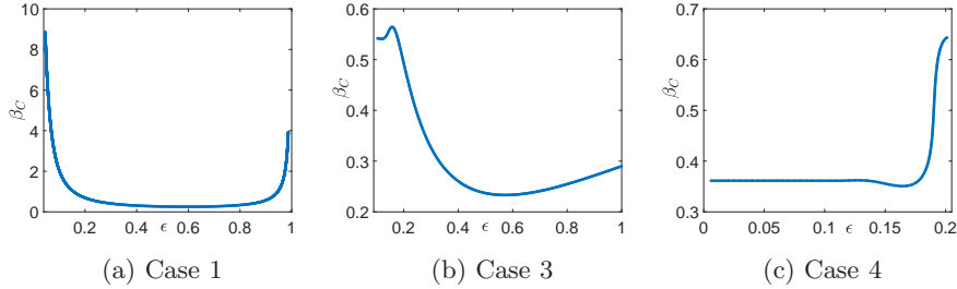
Figure 10: Critical temperature \beta_C as a function of \epsilon for the multiscale Fokker-Planck equation with \theta = 5 for cases (10a) 1 - V^\epsilon(x) = \frac{x^2}{2} + \delta \cos\left(\frac{x}{\epsilon}\right) , (10b) 3 - V^\epsilon(x) = \frac{x^4}{4} - \frac{x^2}{2} + \delta \cos\left(\frac{x}{\epsilon}\right) , and (10c) 4 - V^\epsilon(x) = \frac{x^4}{4} - \frac{x^2}{2} (1 - \delta \cos\left(\frac{x}{\epsilon}\right)) in Table 1.
