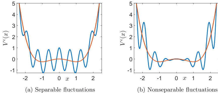
Figure 2: Bistable potential with (left) separable and (right) nonseparable fluctuations.
