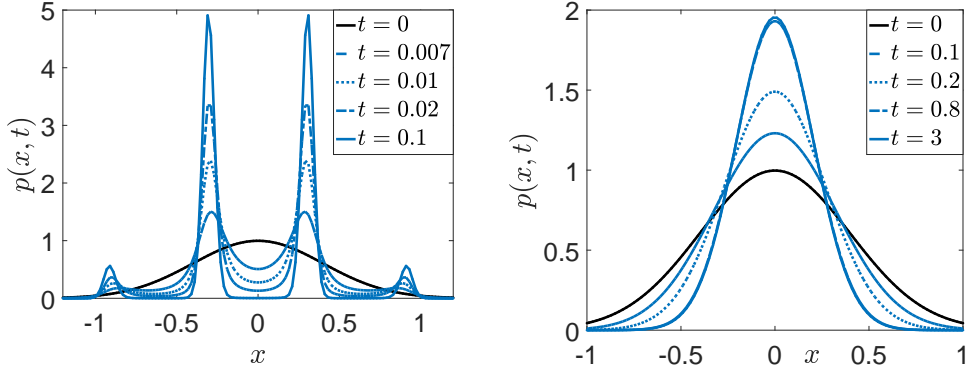
Figure 17: Time evolution of the McKean-Vlasov equation for V^\epsilon(x) = \frac{x^2}{2} + \delta \cos\left(\frac{x}{\epsilon}\right) with \theta = 2 , \beta = 8 , \delta = 1 . Left: (4.6) with \epsilon = 0.1 . Right: homogenized equation (4.7).
