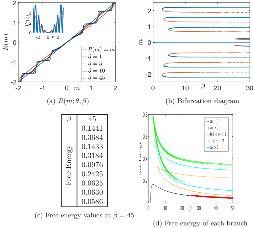
Figure 7: Results for case 2: convex V_0 with nonseparable fluctuations, for \theta = 5 , \delta = 1 , \epsilon = 0.1 . (7a) R(m; \theta, \beta) for various values of \beta , with the potential V^\epsilon(x) (full line) compared with V_0^\epsilon(x) (dashed line) in the inside panel. (7b) Bifurcation diagram of m as a function of \beta . Full lines correspond to stable solutions, while dashed lines represent unstable ones. (7c) Values of the free energy of the steady state in each branch of (7b) for \beta = 45 . (7d) Free energy of each branch of the bifurcation diagram.
