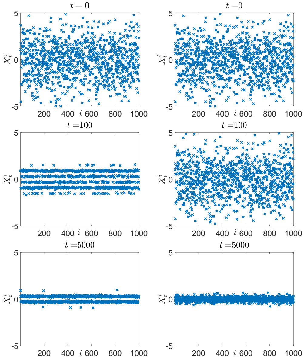
Figure 11: Position of N = 1,000 particles for V^\epsilon(x) = \frac{x^2}{2} + \delta \cos\left(\frac{x}{\epsilon}\right) , with \theta = 2 , \beta = 8 , \delta = 1 . Left: Eqn. (2.1) with \epsilon = 0.1 . Right: homogenized SDEs (2.17).
