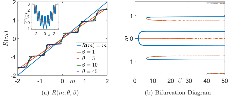
Figure 6: Results for case 1: convex V_0^c with separable fluctuations, for \theta = 5 , \delta = 1 , \epsilon = 0.1 . (6a) R(m^\epsilon; \theta, \beta) for various values of \beta , with the potential V^\epsilon(x) (full line) compared with V_0^c(x) (dashed line) in the inside panel. (6b) Bifurcation diagram of m as a function of \beta . Full lines correspond to stable solutions, while dashed lines represent unstable ones.
