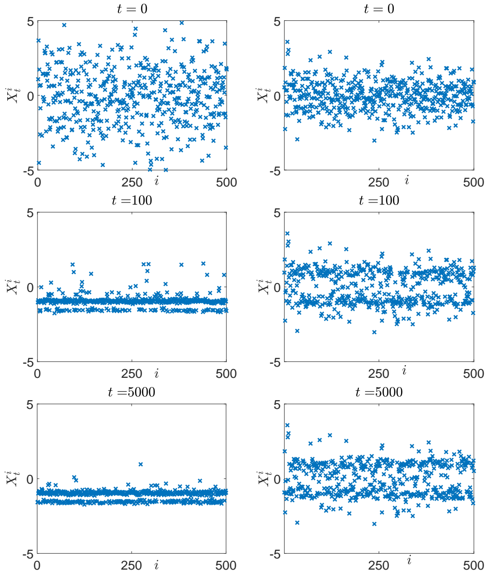
Figure 14: Position of N = 500 particles for V^\epsilon(x) = \frac{x^4}{4} - \frac{x^2}{2} (1 - \delta \cos(\frac{x}{\epsilon})) , with \theta = 0.5 , \beta \approx 5.6 , \delta = 1 . Left: Eqn. (2.1) with \epsilon = 0.1 . Right: homogenized SDEs (2.17).
