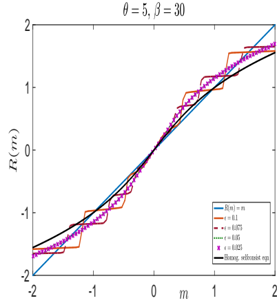
(b) \frac{x^4}{4} - \left(1 + \delta \cos\left(\frac{x}{\epsilon}\right)\right) \frac{x^2}{2}
